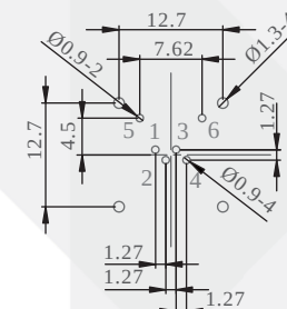
PCB. layout
